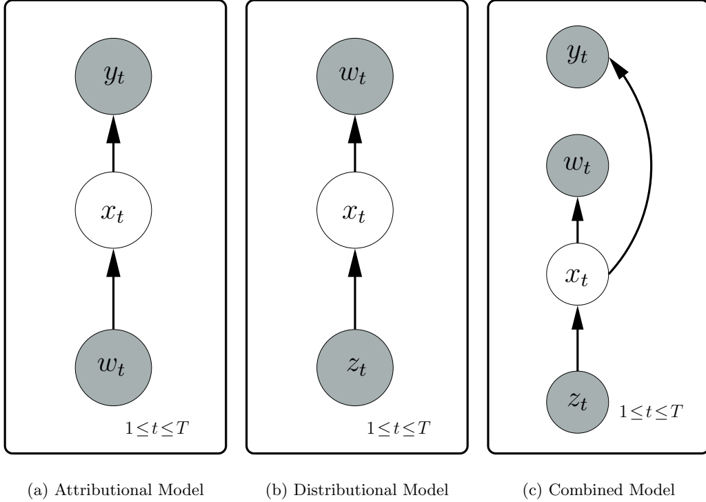
Figure 1: The generative models that utilize a) attributional, b) distributional and c) combined information sources.
